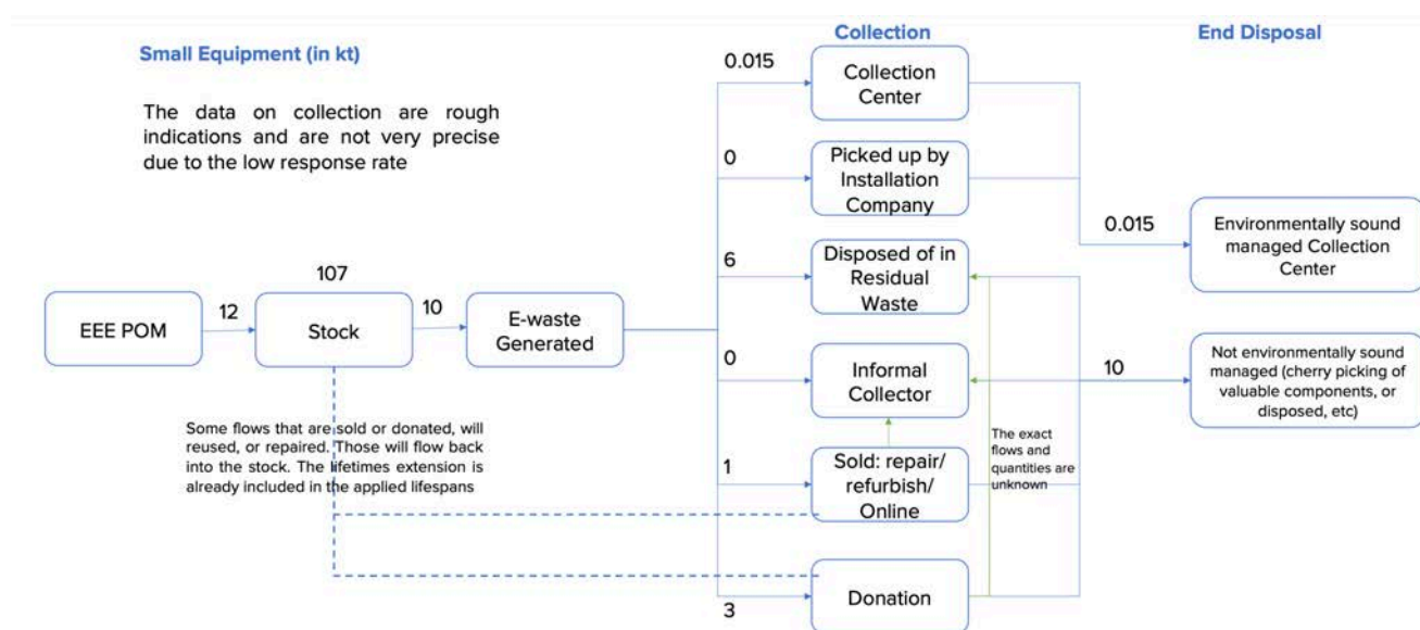
Figure 21 – Mass flows for small equipment
